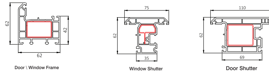
Casement Window
